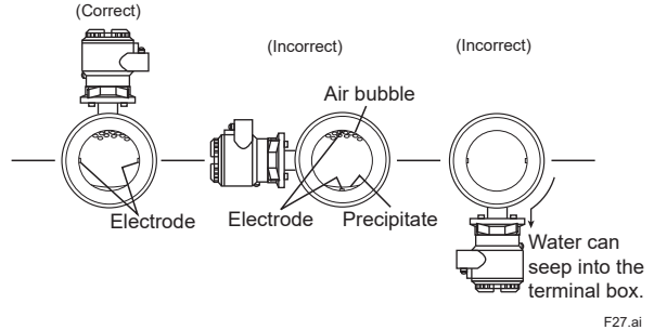
Mounting Orientation
