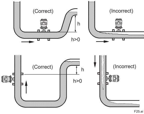
Mounting Positions
